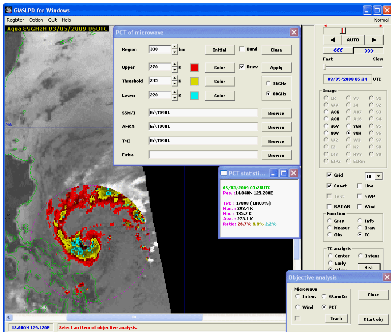
Figure 9.7.5 An Example Drawing Distribution Map of PCT
