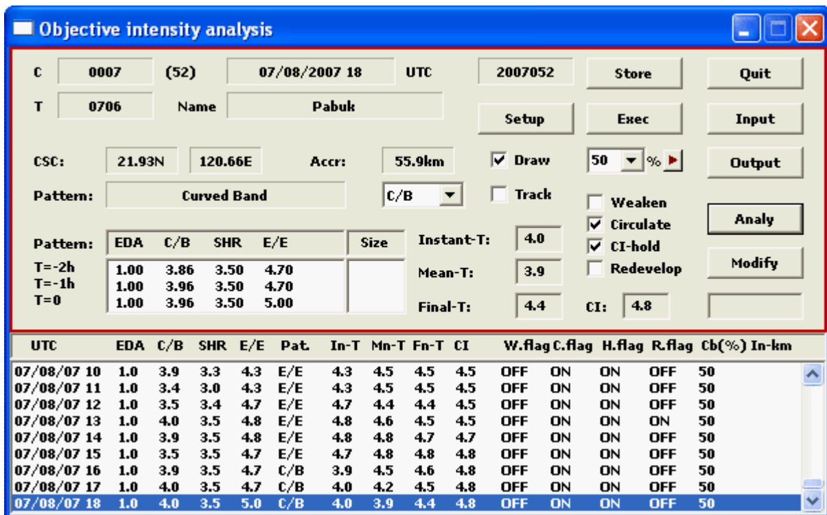
Figure 9.7.1.1 An Example Estimating Objective Intensity of Tropical Disturbance
