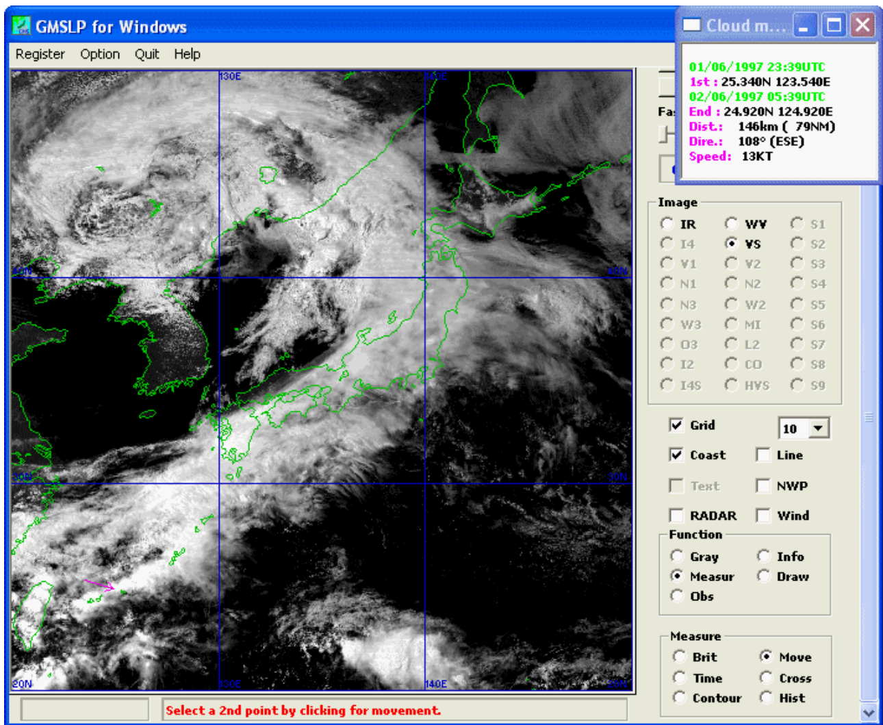
Figure 5.3.3.3 Measurements Based on Visible Images to Indicate the Movement of a Cb Line
