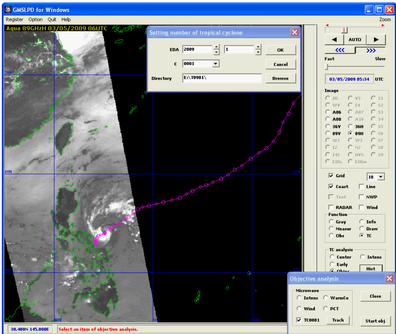
Figure 9.7.6 An Example Drawing Track of Center Positions
