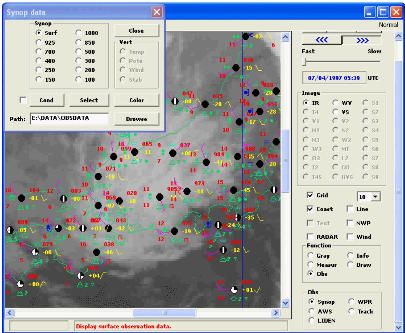
Figure 5.3.5.6 A Satellite Image Synthesized with Synoptic Observation Data (An enlarged view is synthesized with observations of the surface and the marine)
