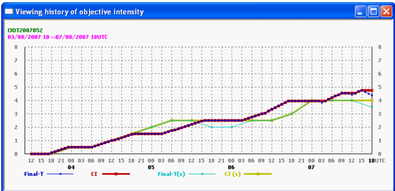
Figure 9.7.1.2 An Example Graphing Objective History of Tropical Disturbance (Subjective History is added.)
