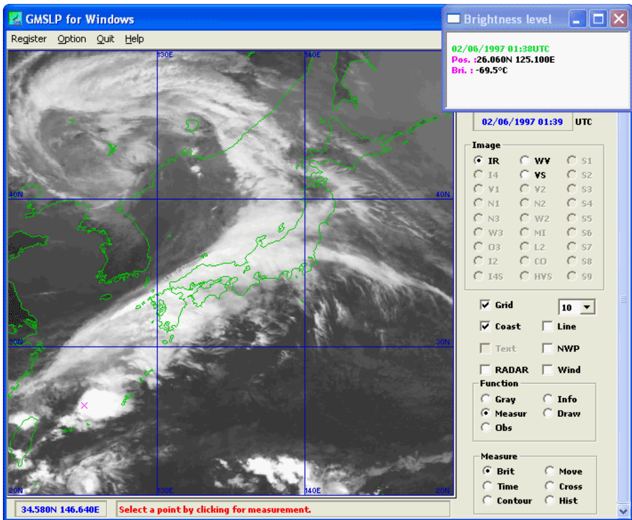
Figure 5.3.3.1 An Example Brightness Temperature Measurement in a Cumulonimbus Area Based on an Infrared Image
