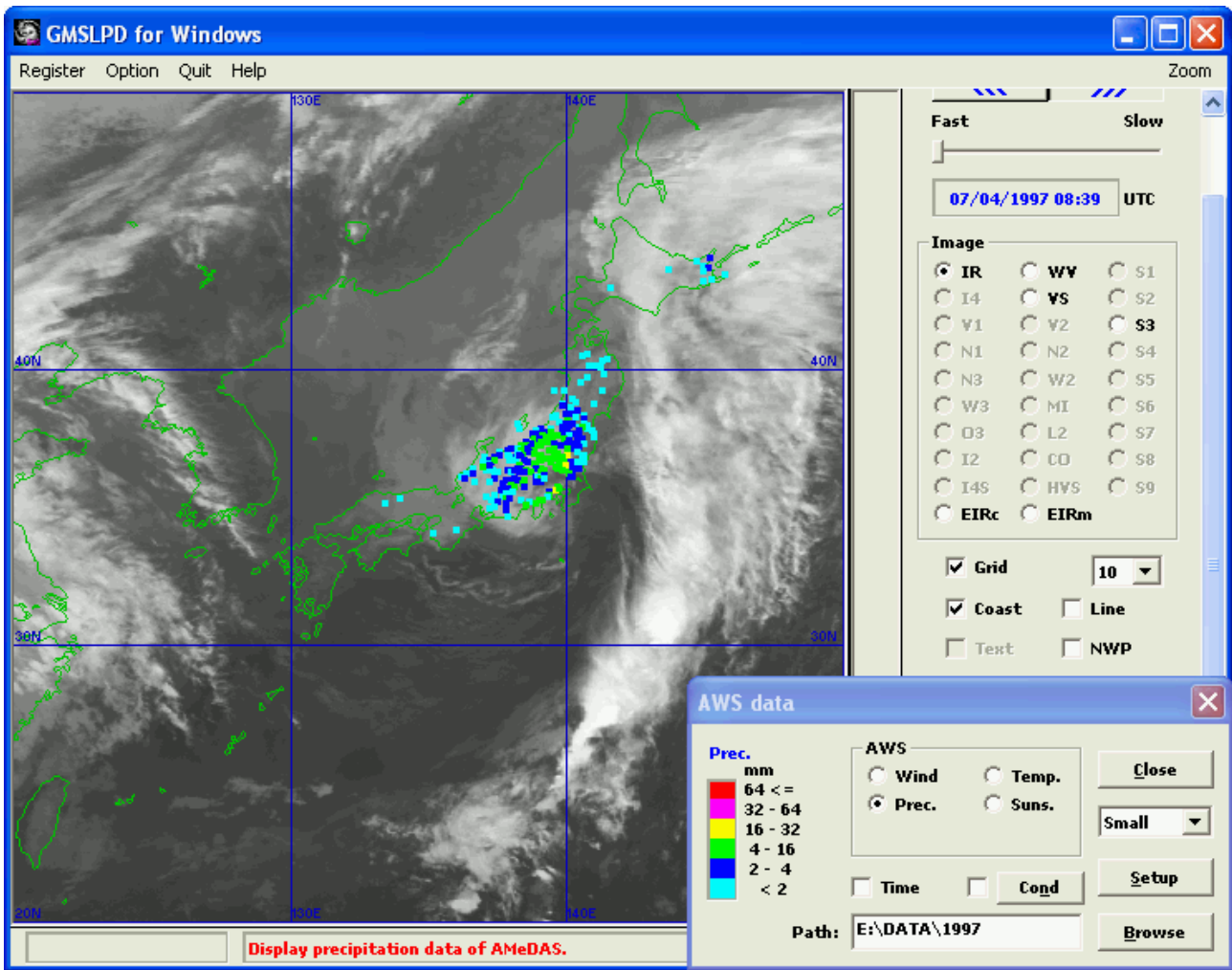
Figure 5.3.5.3 A Satellite Image Synthesized with AWS Data (Precipitation data is synthesized on a normal view)
