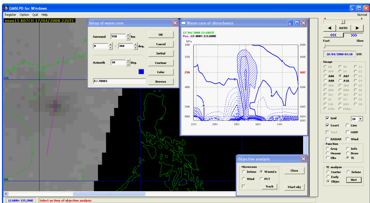
Figure 9.7.3.2 An Example Displaying Cross Section of Warm Core and Setup of Warm Core (The hatch is set where difference of temperature is 1.0 degrees or more.)
