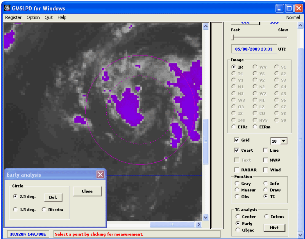
Figure 9.6.1 An Example Discrimination in Early Stage of Tropical Cyclones (The area where brightness temperature is -31^{\circ}\text{C} or less is colored.)
