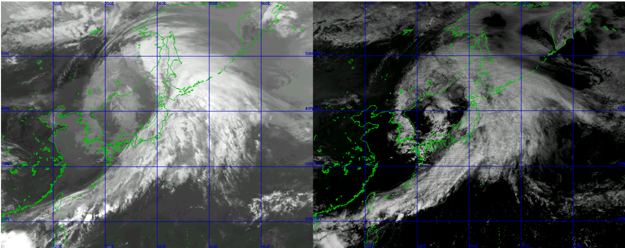
Figure 8.1.2 Comparison Between an Infrared Image (Left) and a Visible Image (Right)
