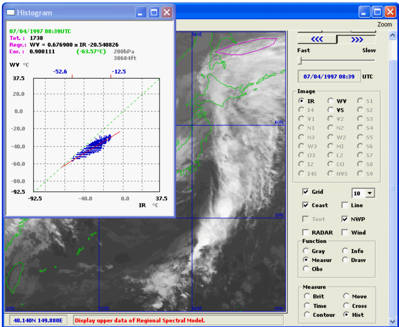
Figure 5.3.3.9 Scattergram of Brightness Temperature Based on Infrared Image and Water Vapor Image
