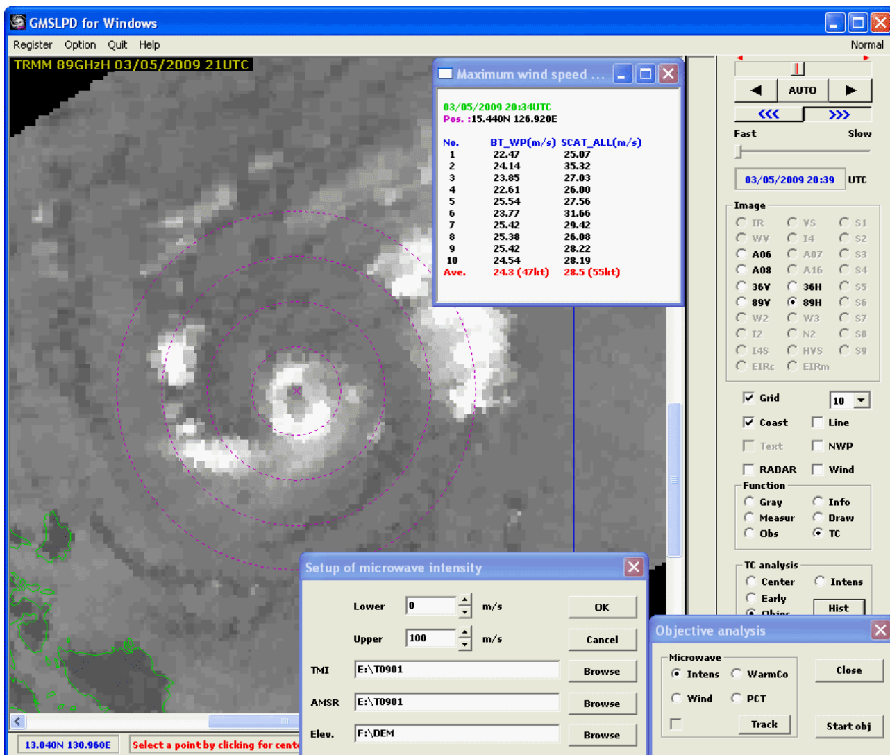
Figure 9.7.2 An Example Estimating Intensity of Tropical Cyclone and Setup of Microwave Intensity
