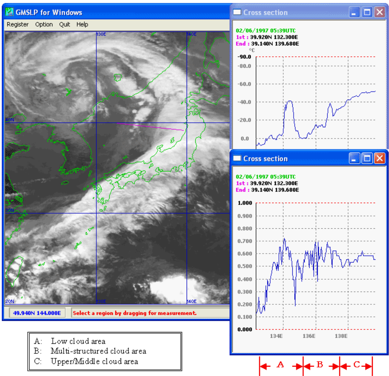
Figure 5.3.3.5 Brightness Distribution Over a Cross Section Upper: Infrared Lower: Visible
