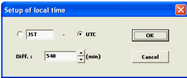
Figure 6.12.2 An Example Setting of the [Setup of local time] Window
