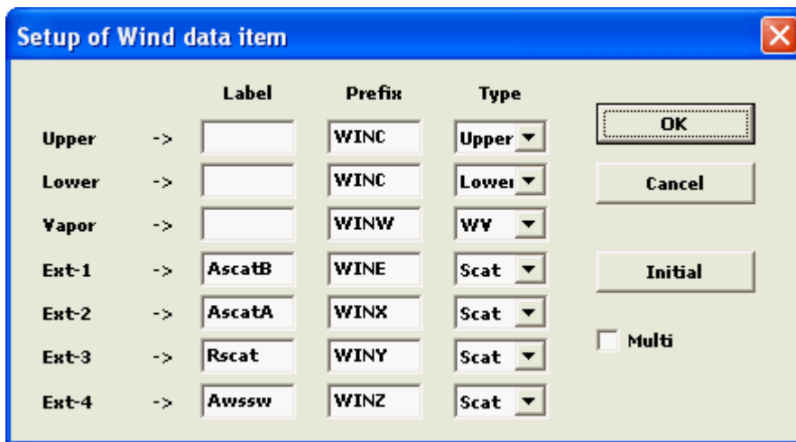
Figure 5.2.5.2 Example Settings of the [Setup of Wind data item] Window
