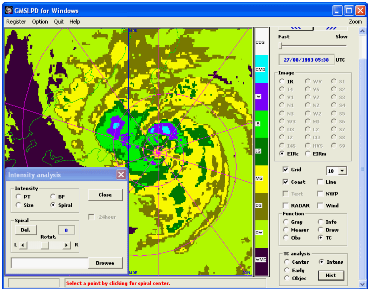
Figure 9.4 An Example of Estimating the Intensity of a Tropical Cyclone (By measuring the length of the cloud band in an enhanced infrared image)
