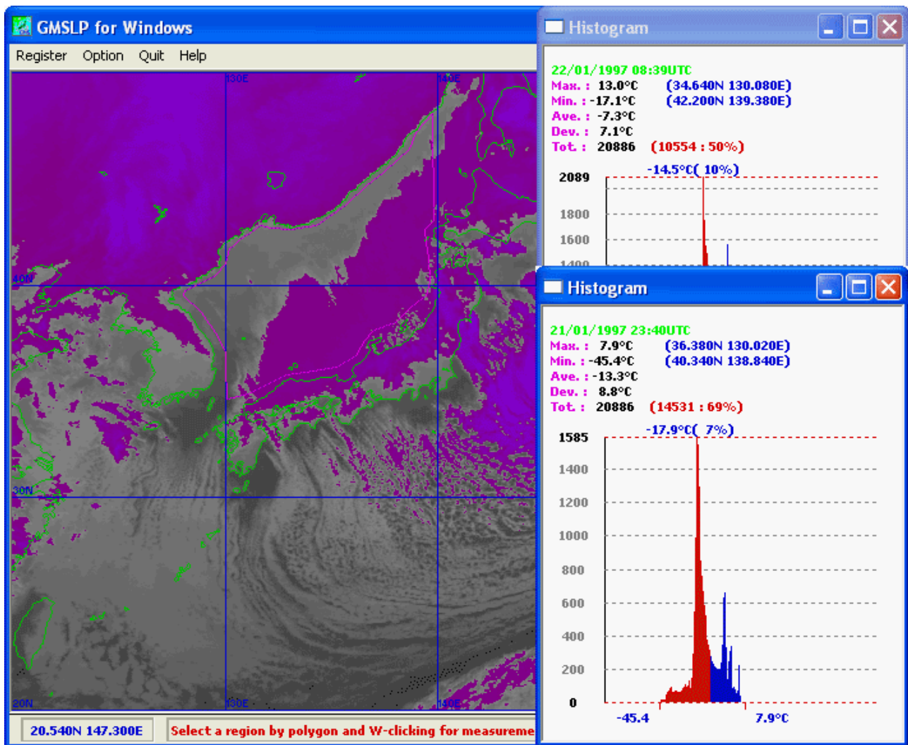
Figure 5.3.3.8 Histograms of Brightness Temperature Based on Infrared Images (A brightness temperature range below -10^{\circ}\text{C} has been emphasized) Upper: 09UTC, Lower: 00UTC
