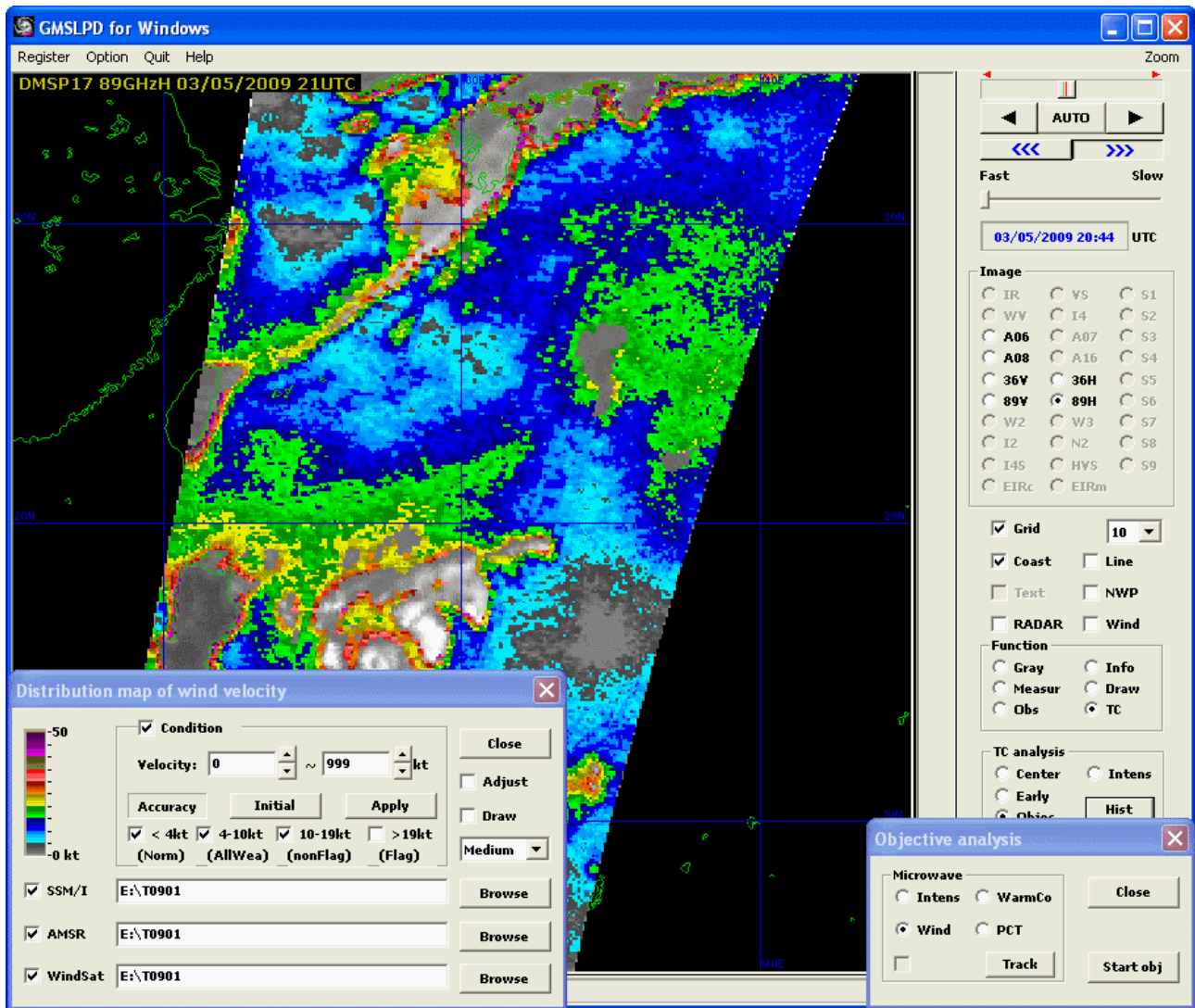
Figure 9.7.4 An Example Drawing Distribution Map of Wind Speed
