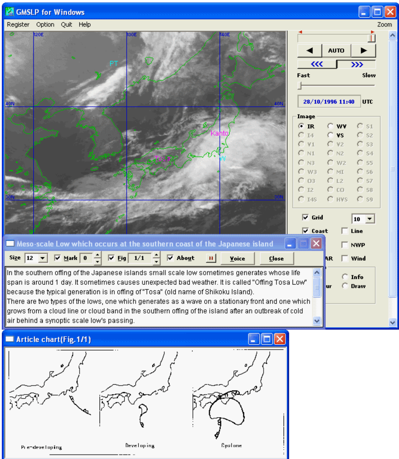
Figure 8.1.5 An Example of the Case Study "A Small low which generates in the south of Japan"
