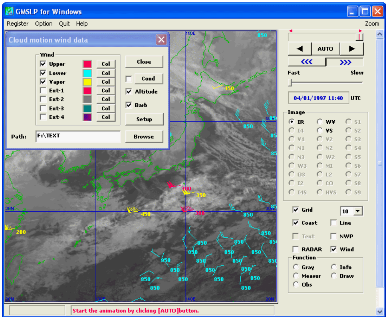
Figure 5.2.5.1 A Satellite Image Synthesized with Cloud Wind Vector Data (The image contains Upper Wind and Lower Wind, Water Vapor Wind, and altitudes)
