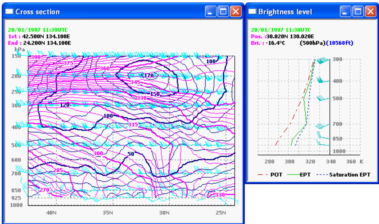
Figure 5.2.4.2 Cross sectional graph (isotachs, wind, and equivalent potential temperature) and vertical profile graph (potential temperature) of NWP data
