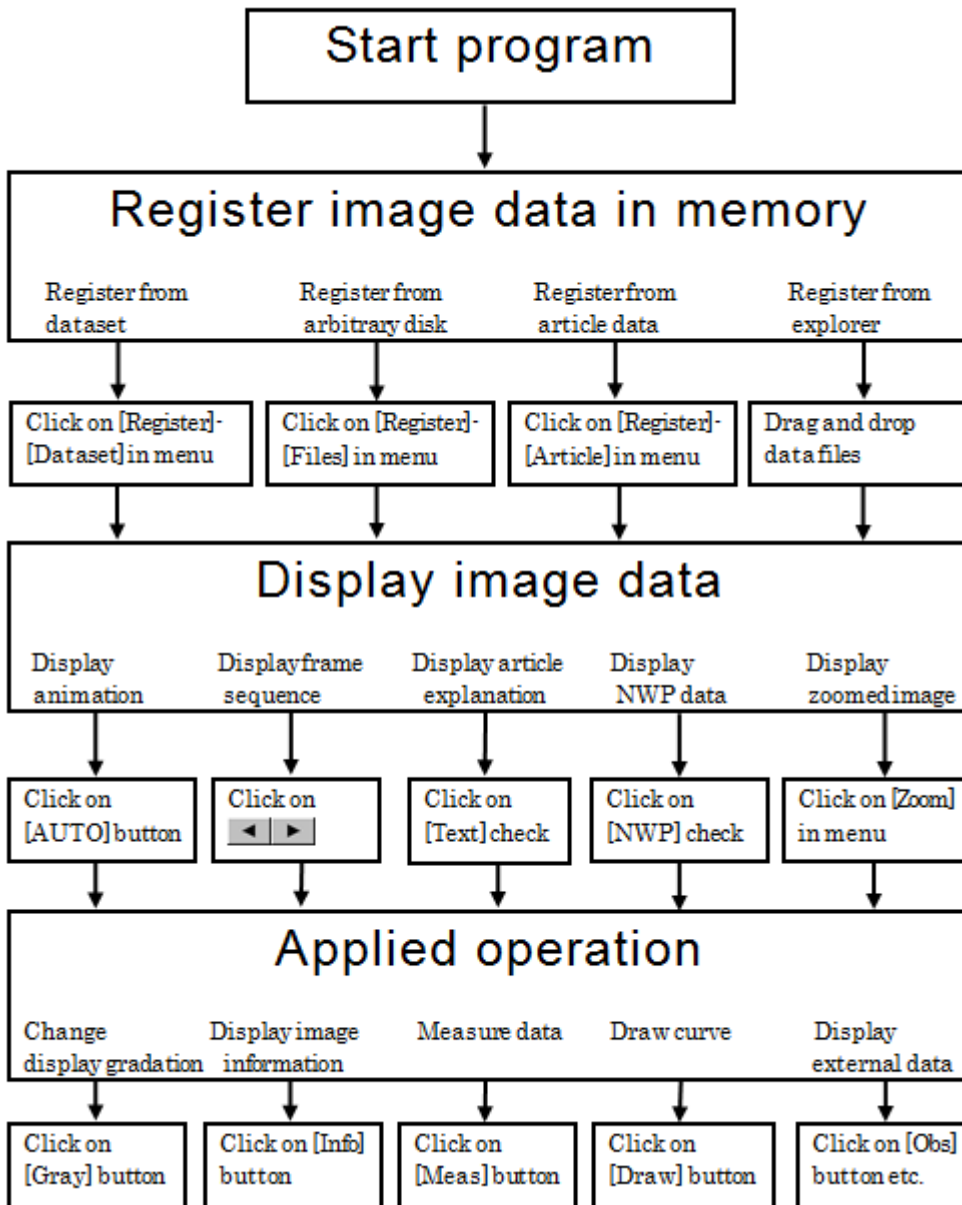
Figure 5.2 Operating Procedures after Starting the Program
