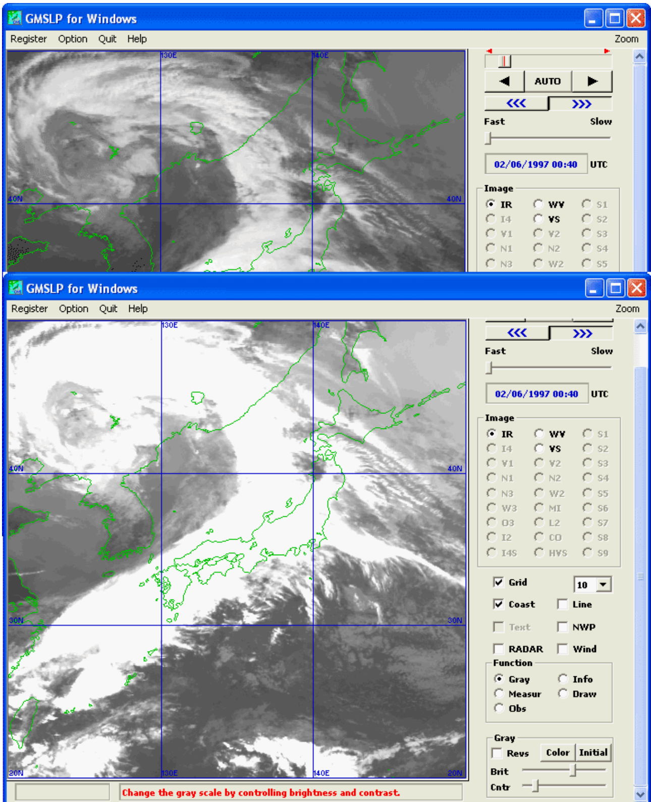
Figure 5.3.1.1 An Infrared Image whose Grayscale has been Changed Upper: Default grayscale Lower: Emphasized low clouds
