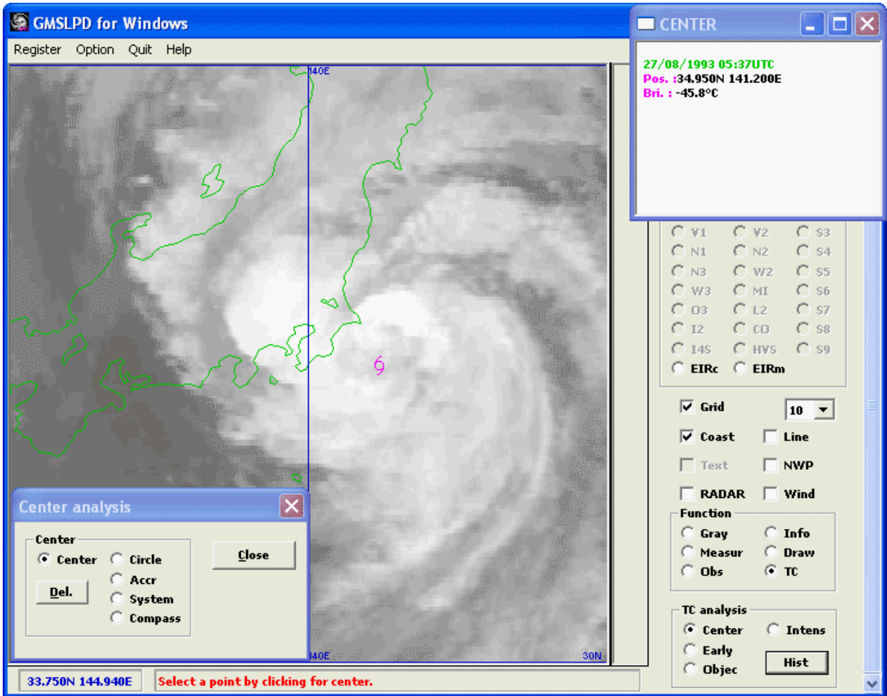
Figure 9.3.1 An Example of Tropical Cyclone Center Analysis
