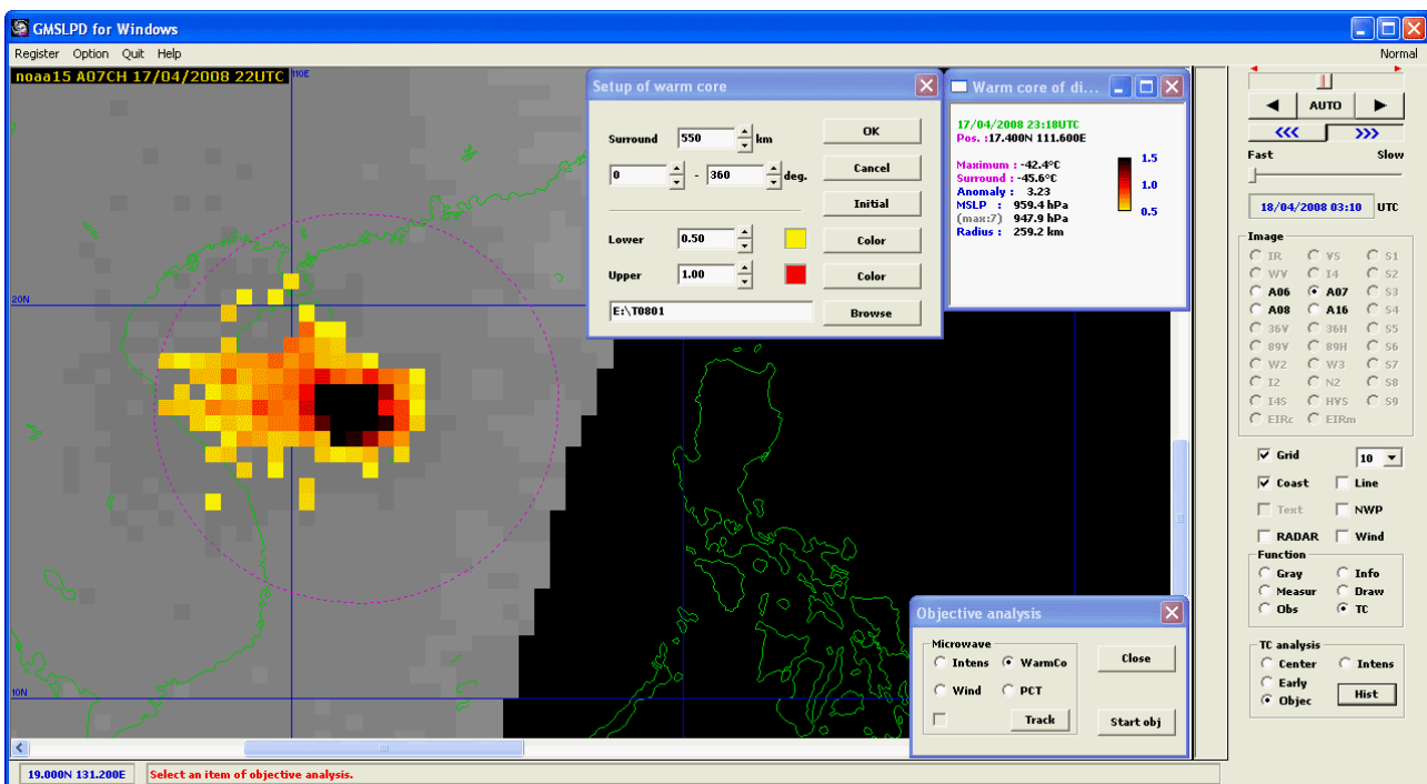
Figure 9.7.3.1 An Example Analyzing Warm Core of Tropical Cyclone and Setup of Warm Core
