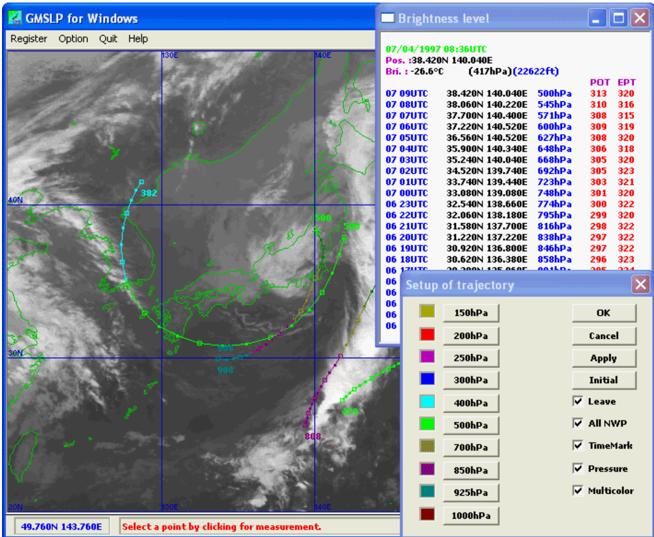
Figure 5.3.3.2 An Example of the Trajectories in an Infrared Image
