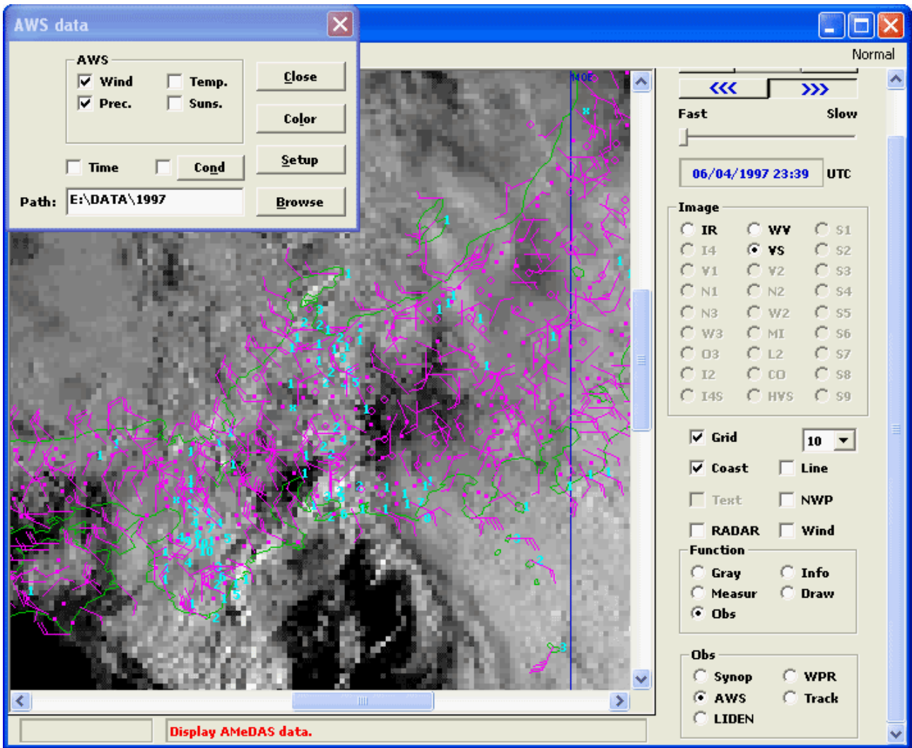
Figure 5.3.5.4 A Satellite Image Synthesized with AWS Data (Wind and precipitation data is synthesized on an enlarged view)
