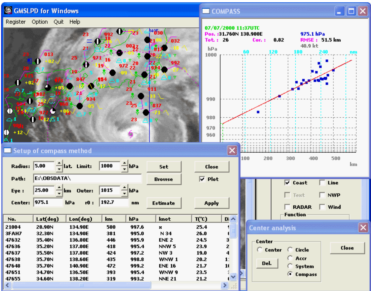
Figure 9.3.2 An Example of Tropical Cyclone Center Analysis by the compass method
