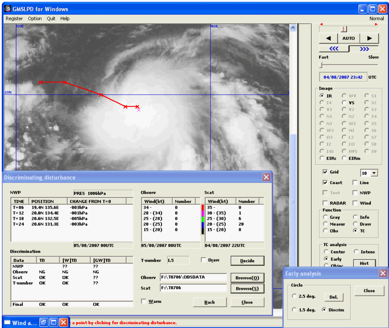
Figure 9.6.2 An Example Discriminating Grade of Tropical Disturbance
