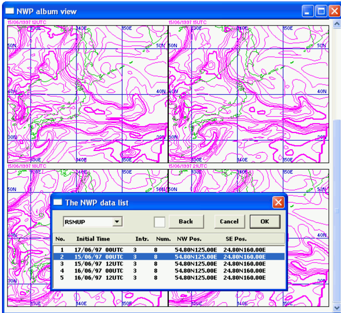
Figure 6.4.3 A List of NWP Data for RSM Upper Air and Example Settings of the [NWP data list] Window
